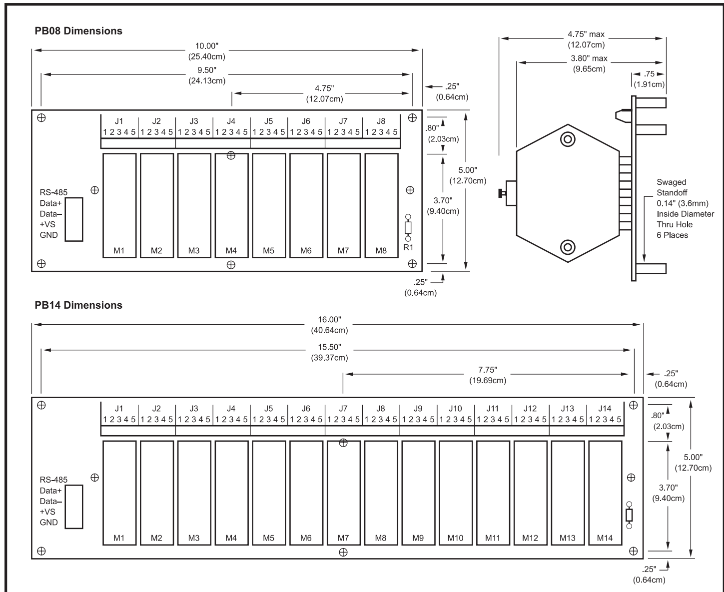
Figure 1: SCM9B-PB08/PB14 Dimensions
